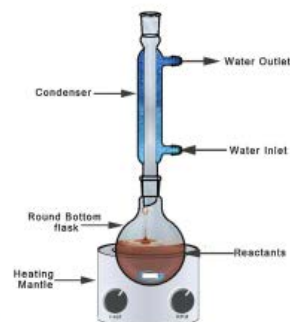
c) Reflux Set Up
